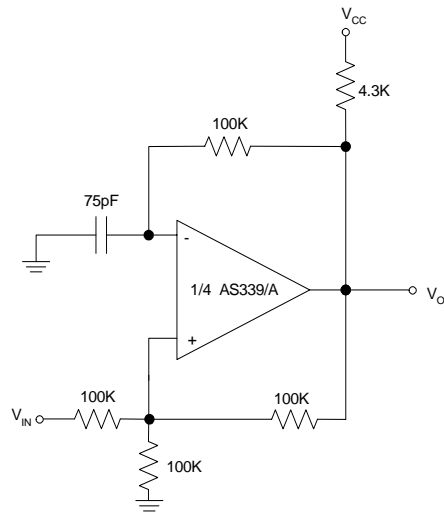
Figure 12. Squarewave Oscillator
